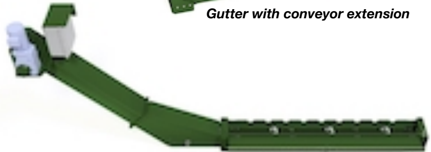
Conveyor drive with gutter extension
