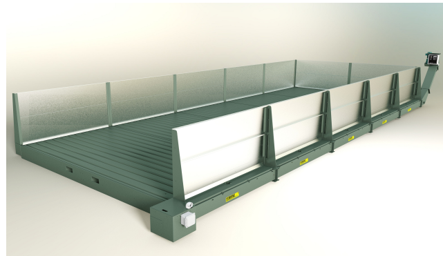
Hydropad wash rack; 16' wide X 40' long, drive on back off design. 4' high walls on 3 sides and drag conveyor for automatic solids removal. Example only.....design exactly what you need.
